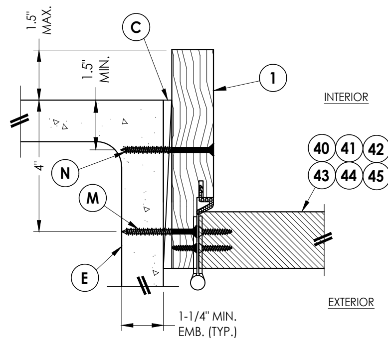
4 HORIZONTAL CROSS SECTION 8 Shown Direct to Masonry Outswing only w/ 6-9/16" jamb
