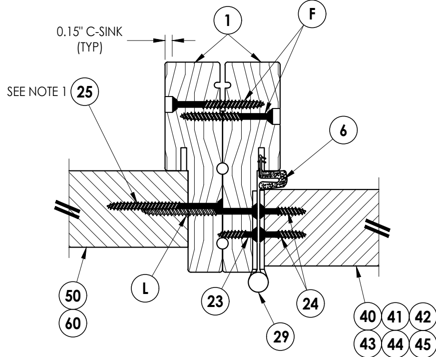
5 HORIZONTAL CROSS SECTION Outswing shown (Inswing similar)
