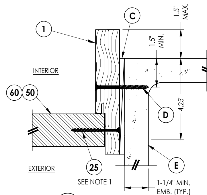
2 HORIZONTAL CROSS SECTION 8 Shown Direct to Masonry Outswing only w/ 6-9/16" jamb
