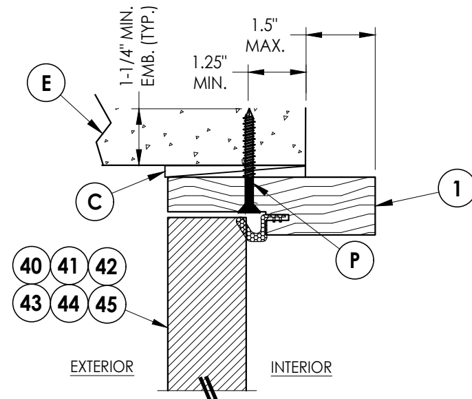
3 VERTICAL CROSS SECTION 8 Shown Direct to Masonry Outswing only w/ 4-9/16" jamb Double Door Only (N/A w/ Sidelites)
