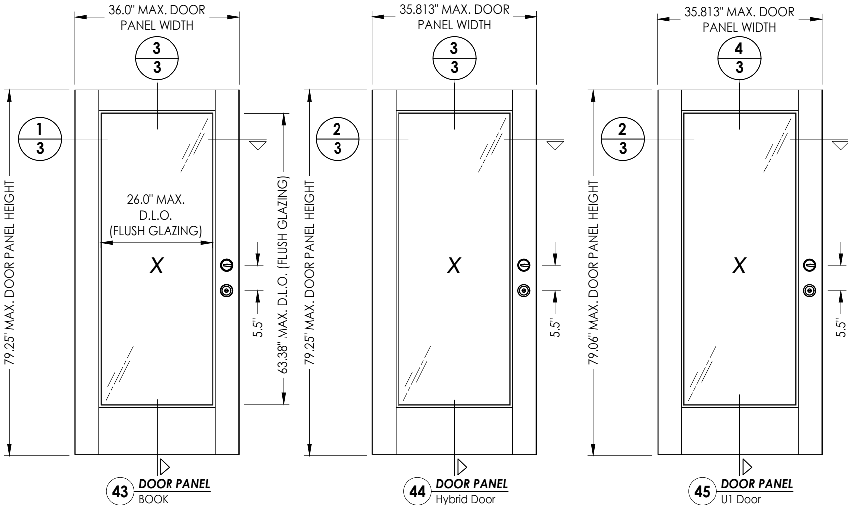
2 HORIZONTAL CROSS SECTION 3 Shown w/ Flush Glazing
