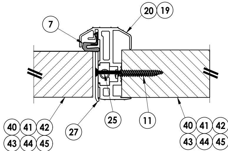
6 HORIZONTAL CROSS SECTION Outswing shown (Inswing similar)
