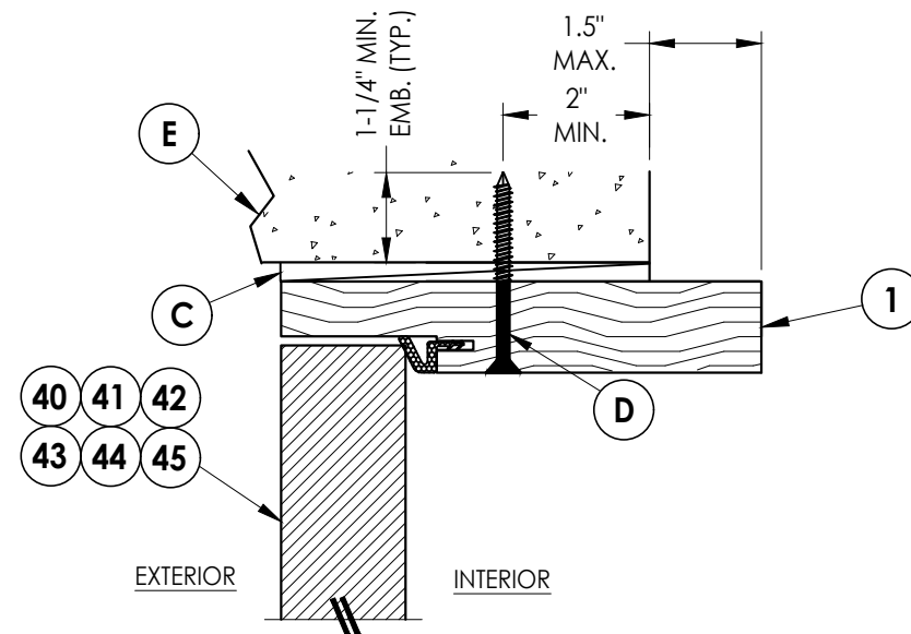
5 VERTICAL CROSS SECTION 8 Shown Direct to Masonry Outswing only w/ 6-9/16" jamb
