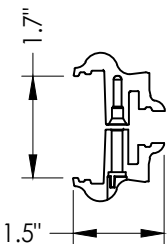
3A BTS LITE FRAME 1/2" & 9/16" Glazing
